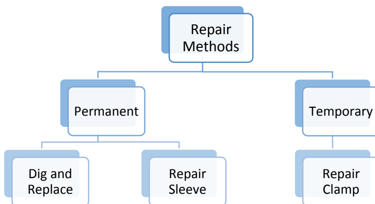
Figure 05.1 Force Main Repair Methods
